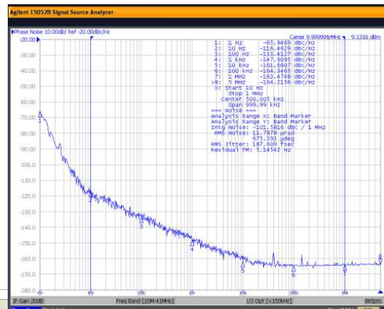
SSB Phase Noise : Square wave(OC13T-10.000)
