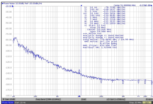
( VC )TCXO with clipped sine wave Test Circuits : Ex. VM14S3
