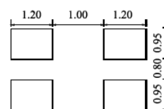
Recommended Solder Pattern
